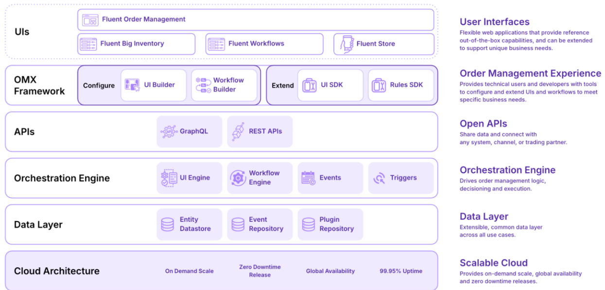
Figure 1: Fluent Order Management System Key Components
